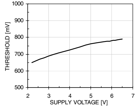
Enable Voltage Threshold
