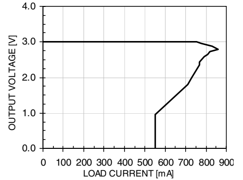
Foldback Current Limiting
